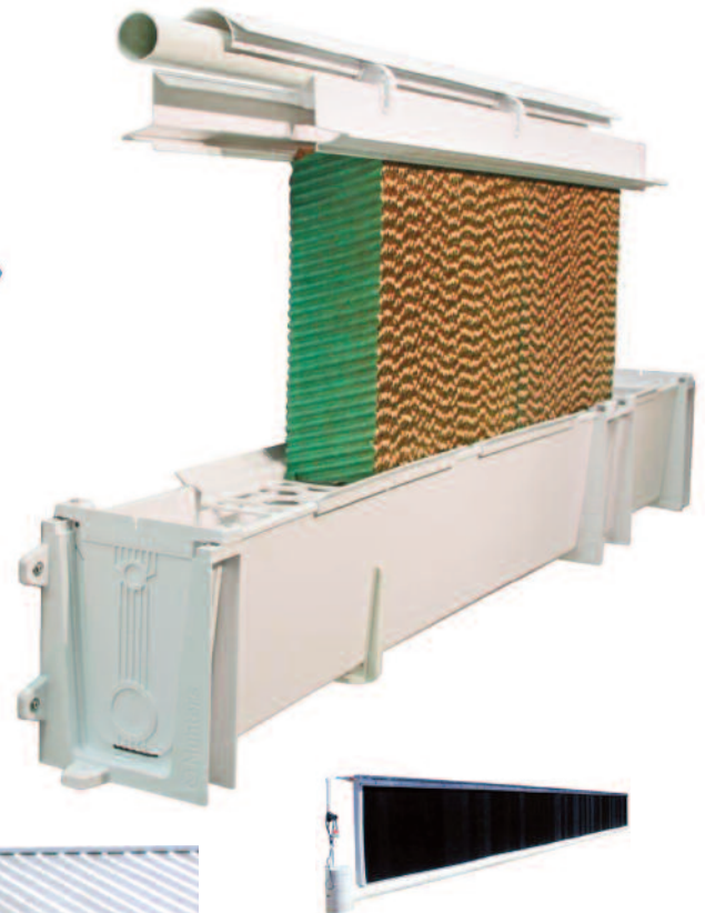
PRINCIPLE OF EVAPORATIVE COOLING.
